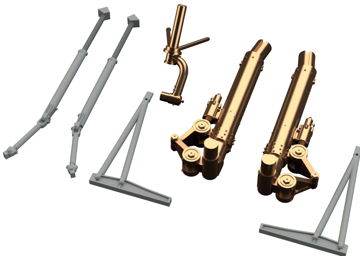
648540 B-17G undercarriage legs BRONZE 1/48 HKM
