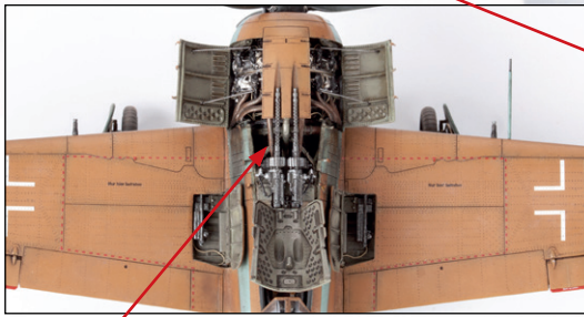
648355 Fw 190A-4 engine & fuselage guns (Brassin)
