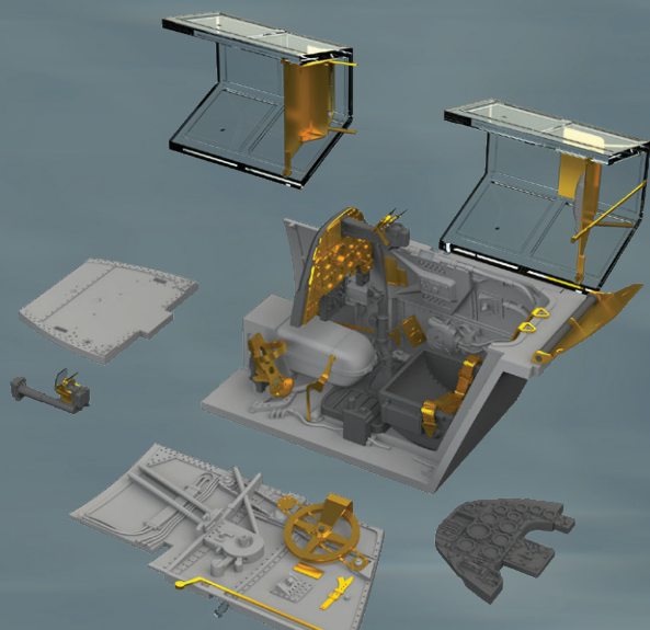
648411 Bf 109G-6/U4 cockpit 1/48 Tamiya
