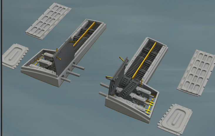
648397 P-51D gun bays 1/48 Airfix
