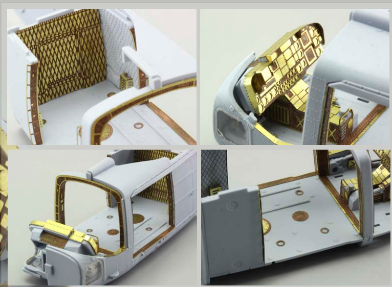
Lynx Mk.88 interior S.A. 1/48 Airfix (49625)
