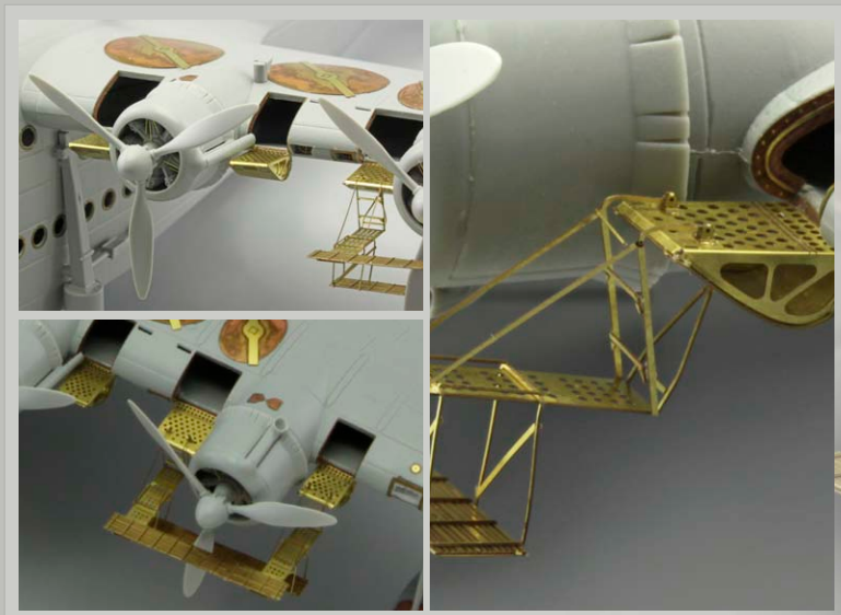
Sunderland Mk.I maintenance platforms 1/72 Italeri (72554)
